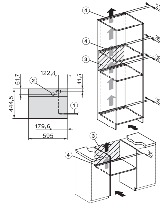
Installation DG DGM, Skizze
